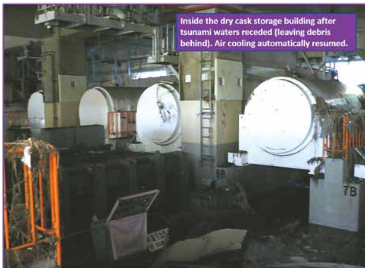
Figure 1.2. Dry cask spent fuel storage at Fukushima. Water initially flooded this chamber, but once the water receded, air cooling resumed. An example of what can go right with dry cask storage. (Source: Union of Concerned Scientists.)
